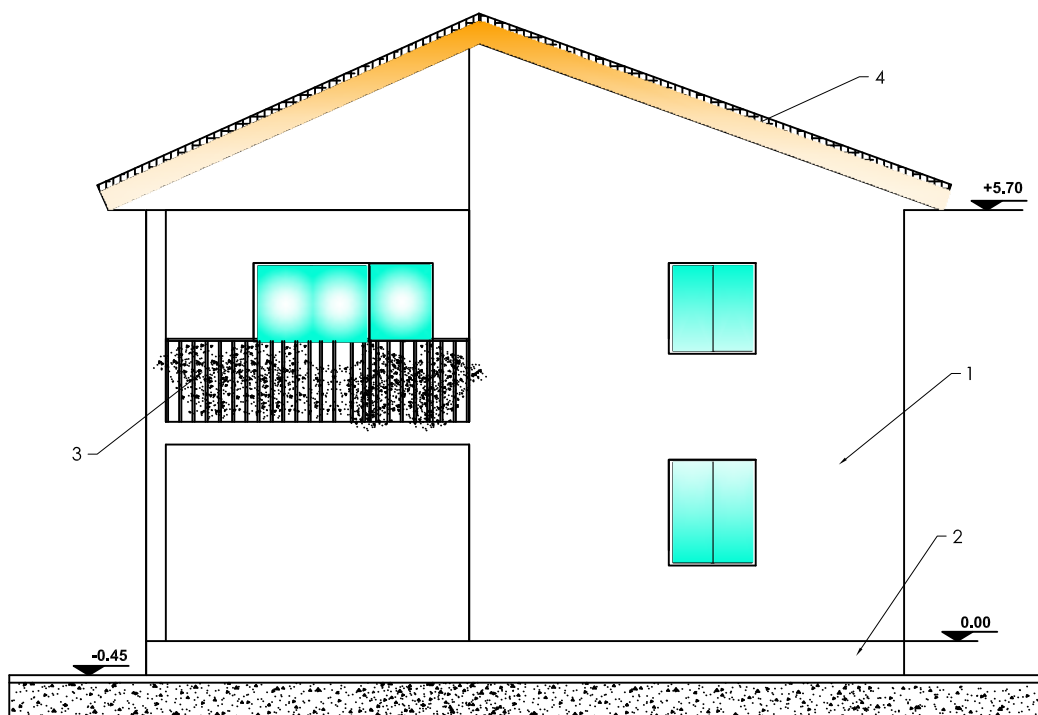
Fatada Vest
